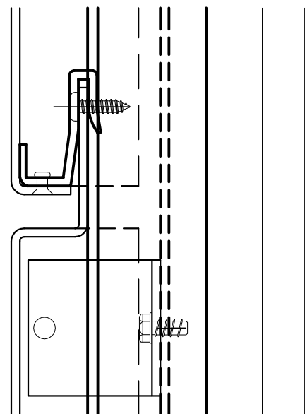
4 1 TYPICAL HORIZONTAL FULL-DEPTH RAIN SCREEN
