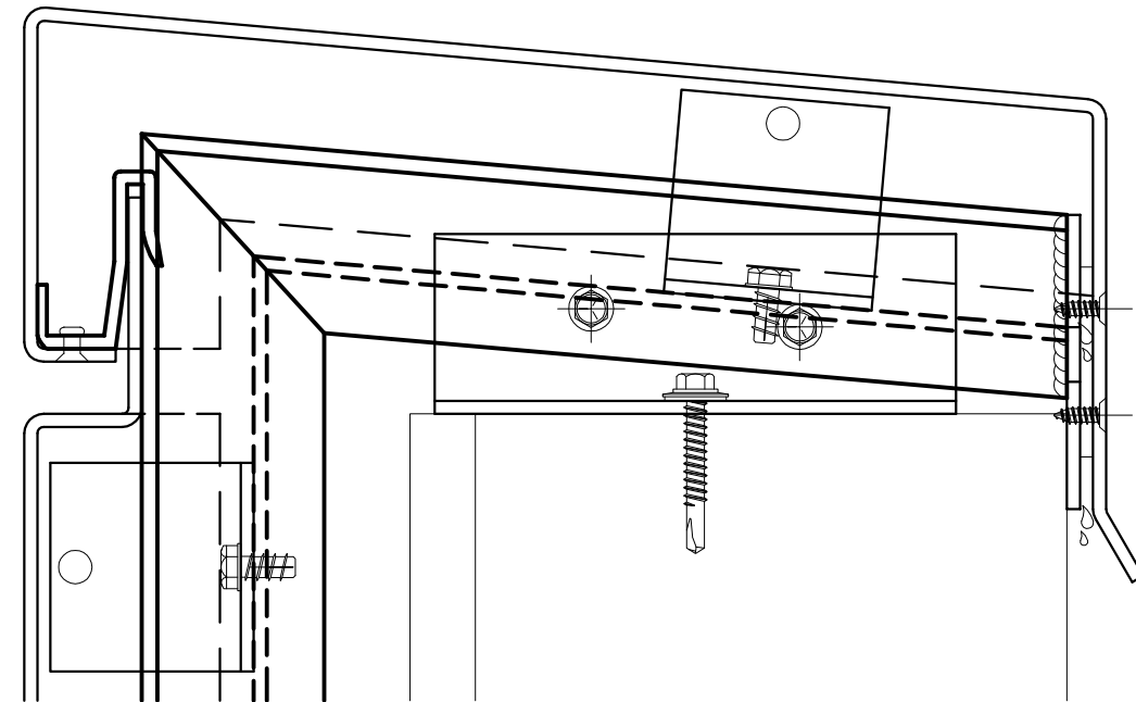
2 1 HORIZONTAL AT COPING FULL-DEPTH RAIN SCREEN
