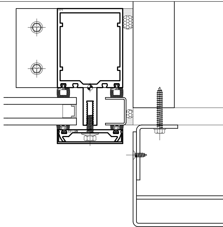
1 1 VERTICAL AT WINDOW JAMB FULL-DEPTH RAIN SCREEN
