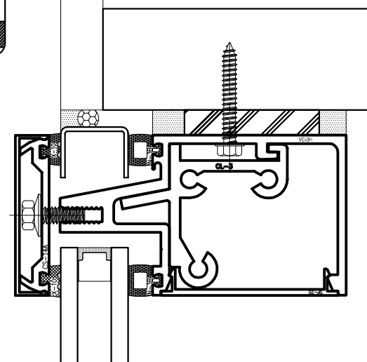
5 1 HORIZONTAL AT WINDOW HEAD FULL-DEPTH RAIN SCREEN
